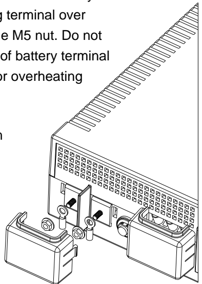
Figure 4 Battery Cable Connection to Inverex
